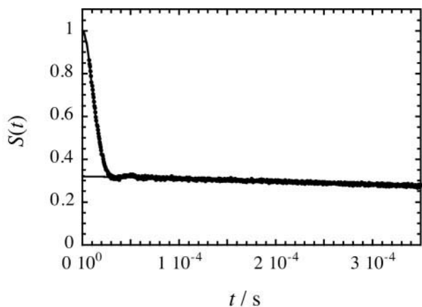
FIGURE 3 Experimental free induction decay obtained on a wet wood pulp fiber sample at -4.6^{\circ}\text{C} . Points, experimental; lines, fitted. The line intersecting the y -axis at 0.32 represents the extrapolation of the water signal to zero time. This value is used for the quantification of the amount of nonfreezing water.
